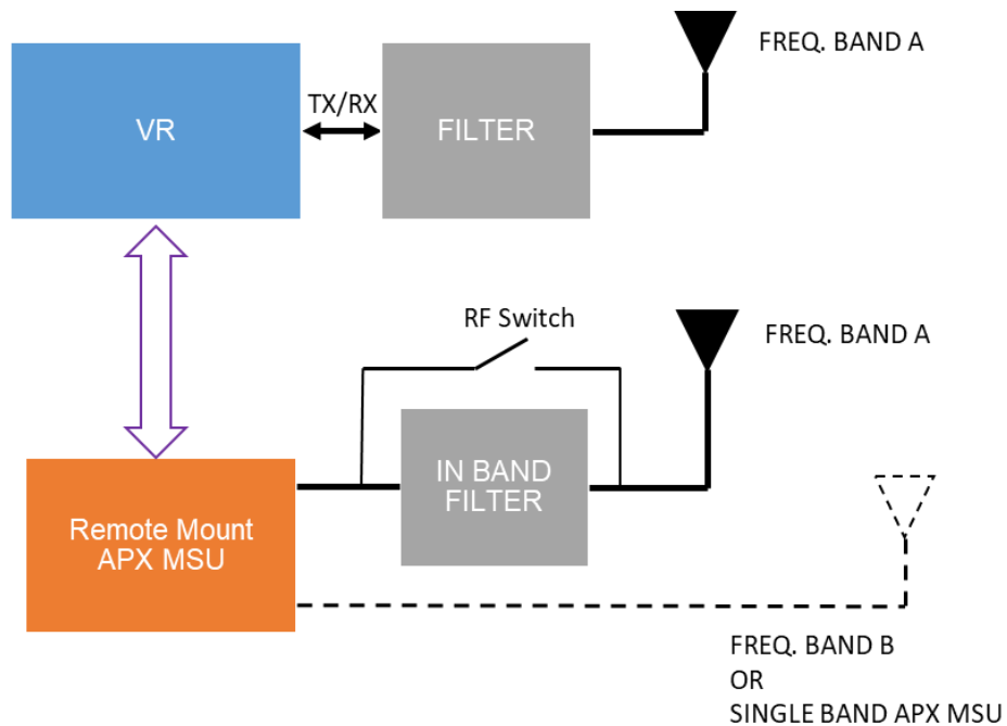
Figure 2 In-Band DVR / DVR-LX - Conceptual Diagram
