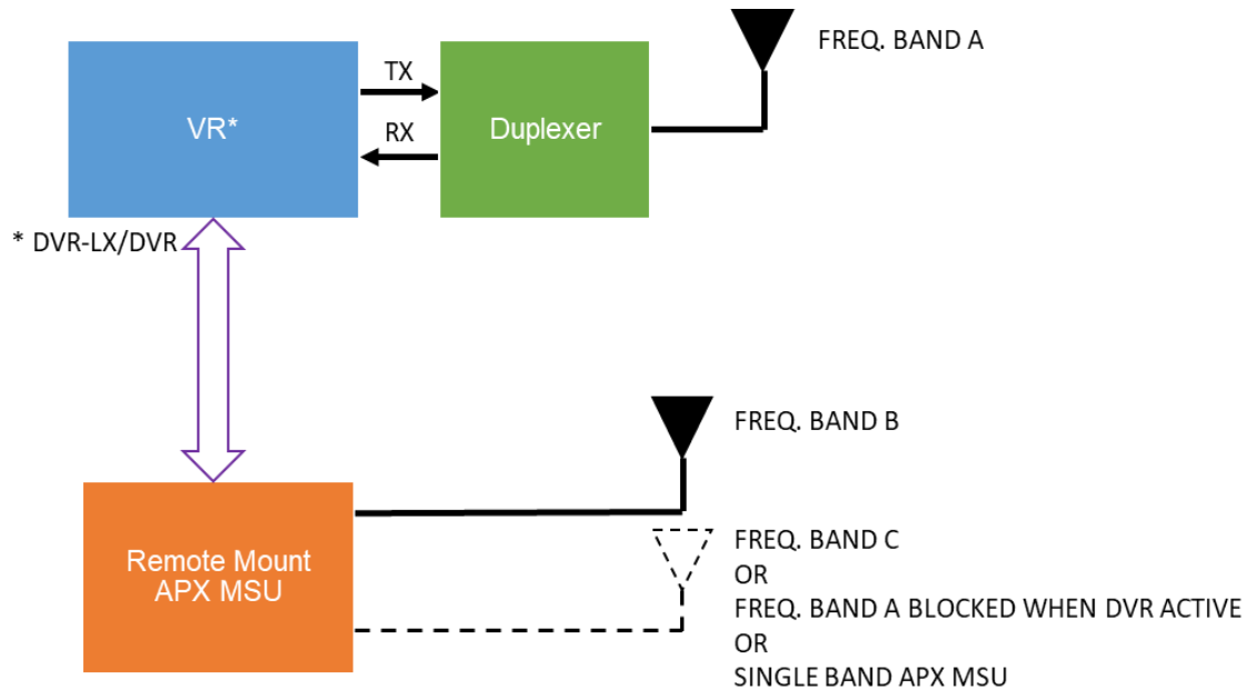
Figure 6 Cross-Band DVR / DVR-LX - Conceptual Diagram
