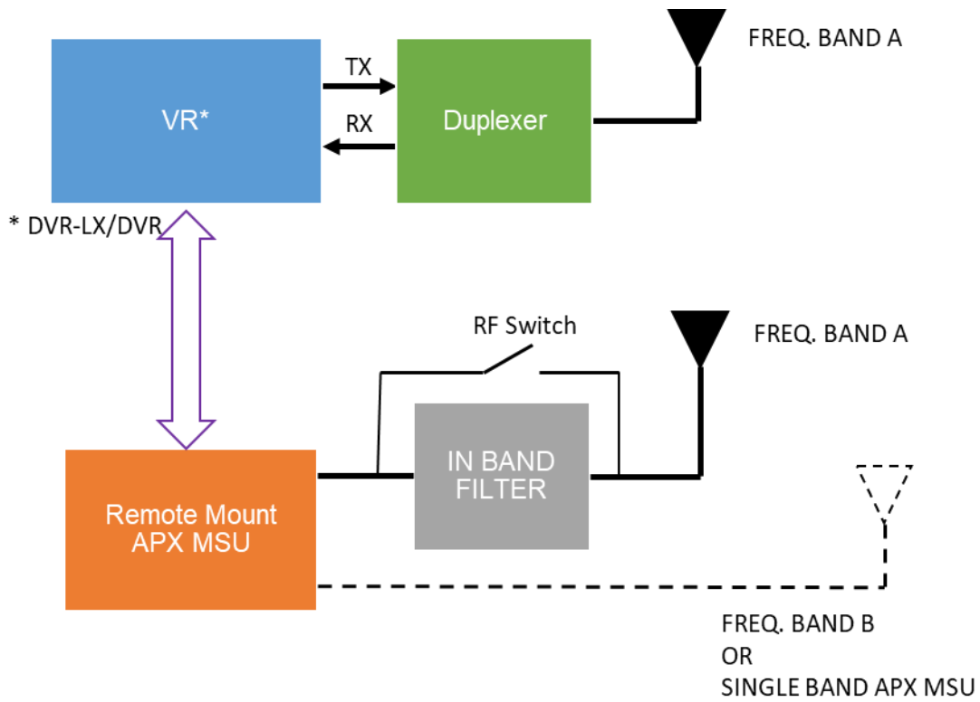
Figure 2 In-Band DVR / DVR-LX - Conceptual Diagram
