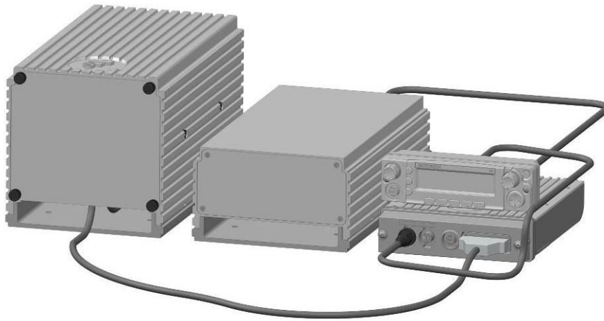
Figure 4 Vehicular Mount In-Band 700 or 800MHz DVRS Model - Full Duplex & Simplex Capable
