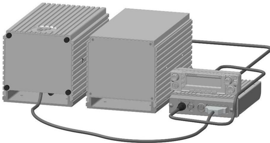
Figure 5 Vehicular Mount In-Band VHF or UHF DVRS Model - Full Duplex & Simplex Capable
