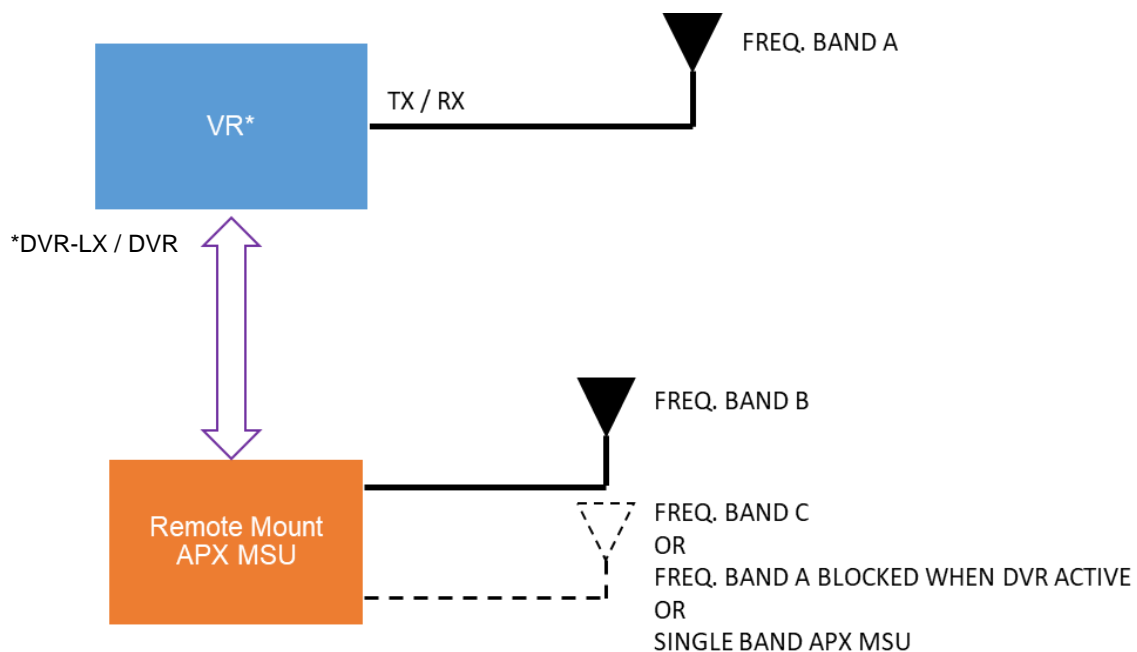
Figure 7 Cross-Band Simplex DVR-LX / VRX1000 - Conceptual Diagram
