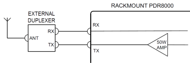
Figure 16: External duplexer with 50W Power Amplifier Hardware Topology
