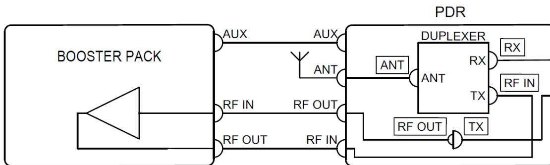
Figure 7: Internal Duplexer and Booster Pack Hardware Topology
