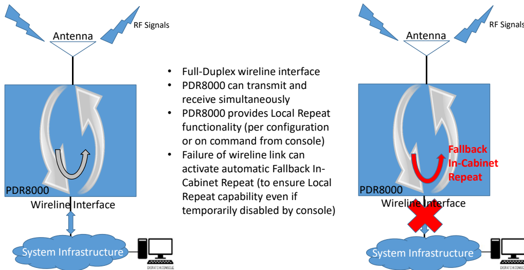
Figure 23: Repeater with Infrastructure Example
