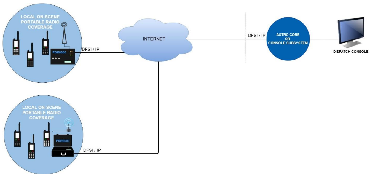
Figure 18: Ethernet Wireline Repeater and Base Station Use Case
