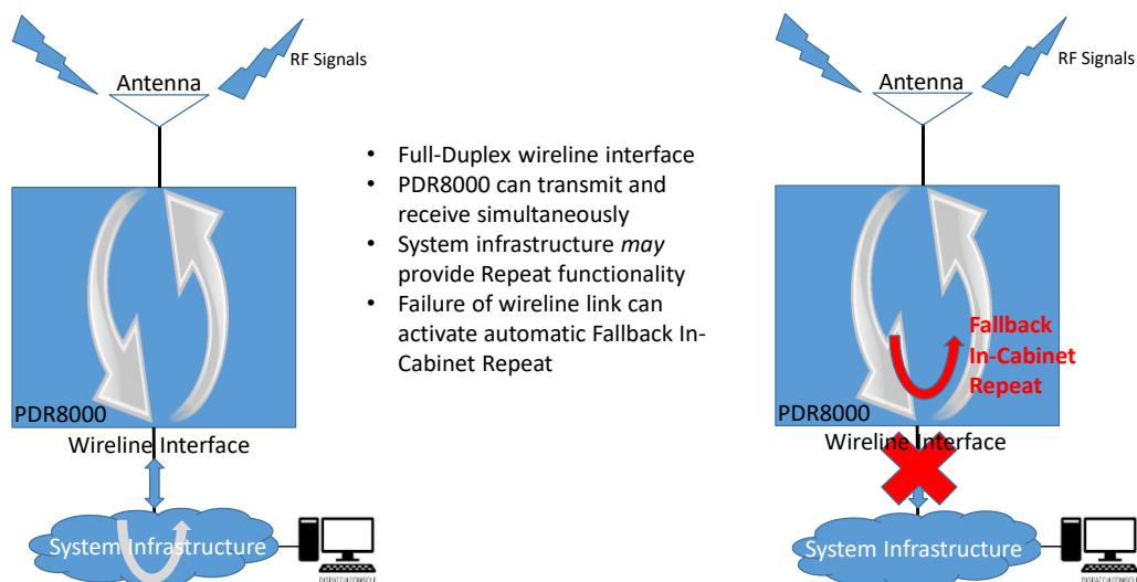
Figure 22: Full-Duplex Base Station Example
