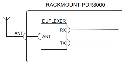
Figure 13: Internal Duplexer Hardware Topology
