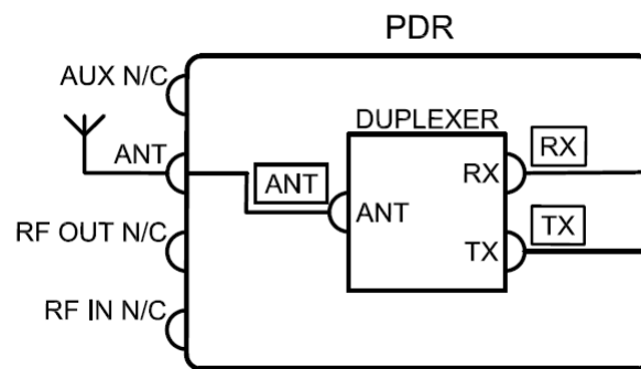
Figure 4: Internal Duplexer Hardware Topology
