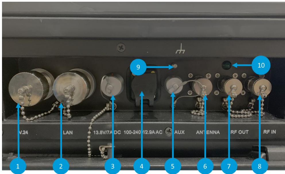
Figure 30: PDR8000 External Ports
