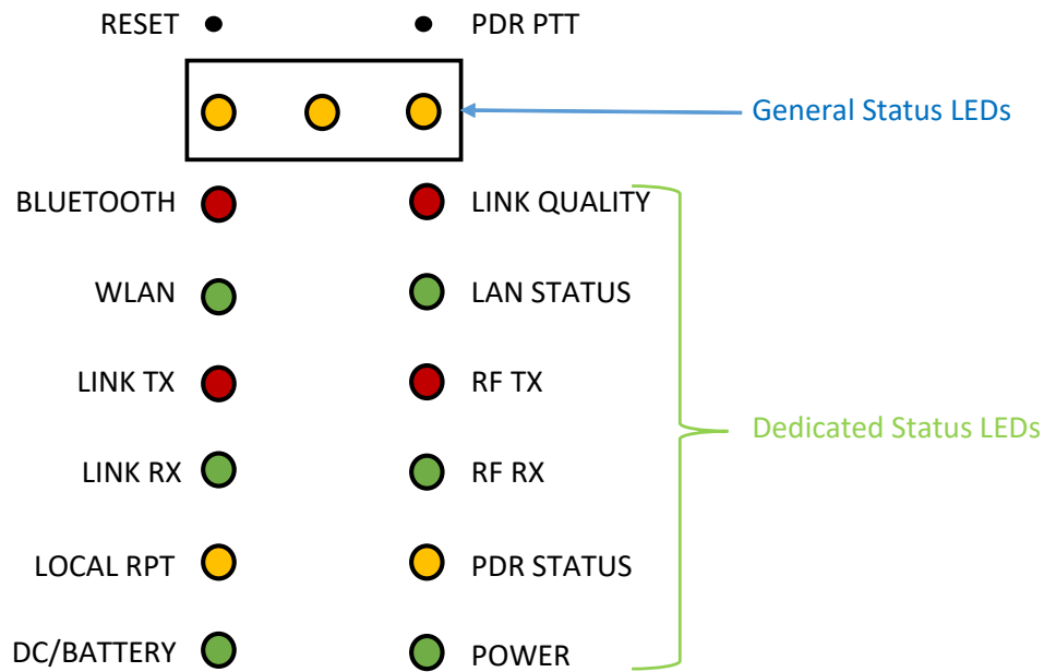
Figure 25: Front Panel LEDs and Switches
