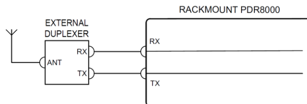
Figure 15: External Duplexer Hardware Topology
