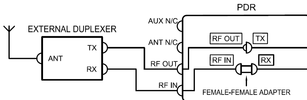
Figure 8: External Duplexer Hardware Topology
