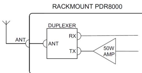
Figure 14: Internal duplexer with 50W Power Amplifier Hardware Topology
