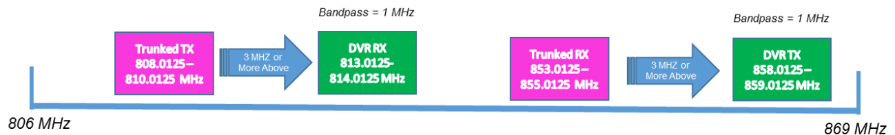
Figure 11 – Scenario 1- 800 MHz DVRS 3 MHz Above Trunked Frequencies with a 1 MHz Band Bandpass
