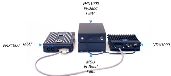
VRX1000 Optional Stacked Mount Configuration
