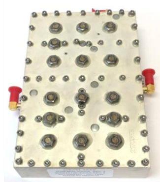
Figure 8: In-Band Filter Duplexer
